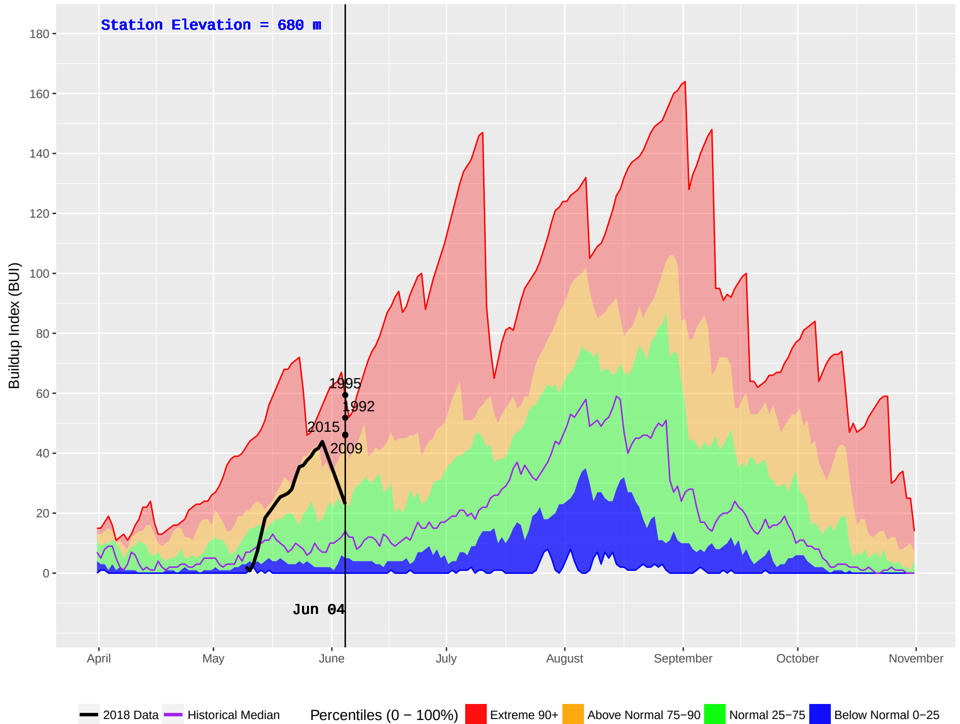
SUMMIT (11) : Historical (1985–2016) and Current (2018) Noon Buildup Index (BUI)
